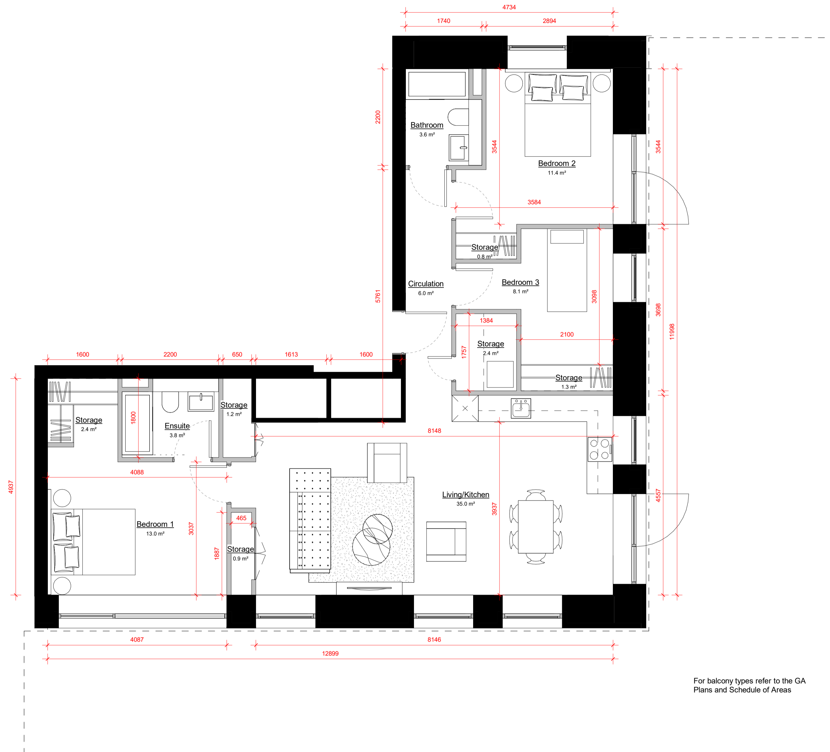
Apartment Type C.7.0 1 : 50
